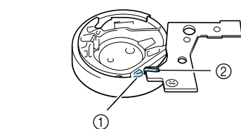
① Projection ② Spring
